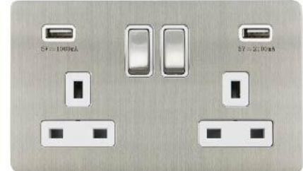
FN270DMF 13A 2G SP Switched Socket + 2 x USB Outlets, Total 3.1A output
